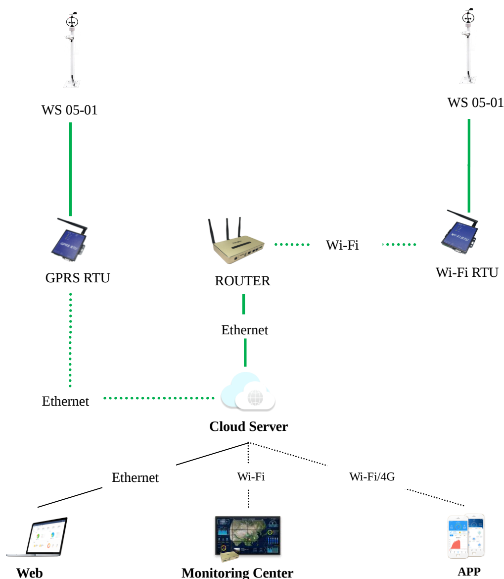
WS 05-01 Product typical networking scheme
